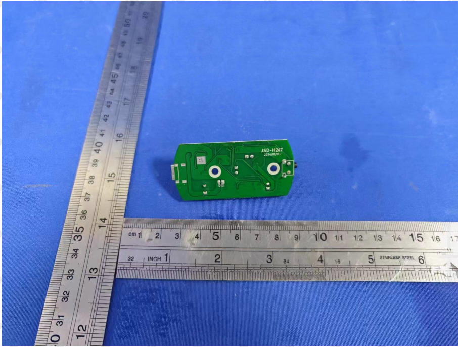
Photo 7: PCB view
